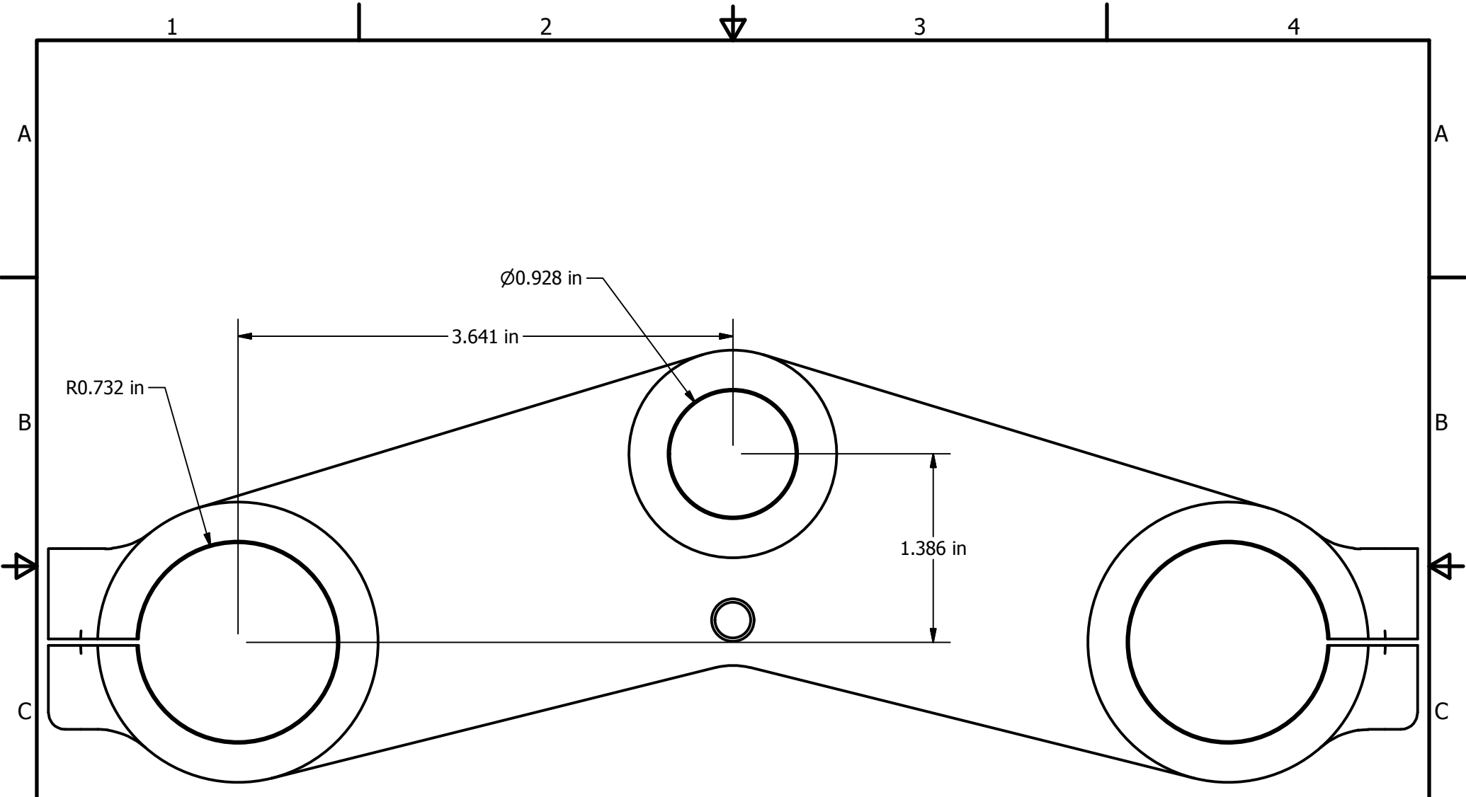
VIEW1: tripple-tree-v3_1 SCALE 1
